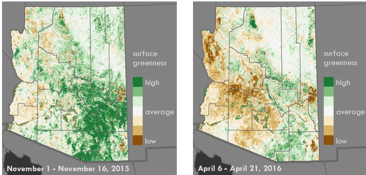
Figure 5. Satellite-measured surface greenness declined between November and April, suggesting that the lack of rain and snow in recent months has curtailed plant growth and reduced plant moisture levels, particularly in the northwestern and southwestern parts of the state 15 . Desiccated vegetation can worsen wildland fire conditions during the April-June fire season.
