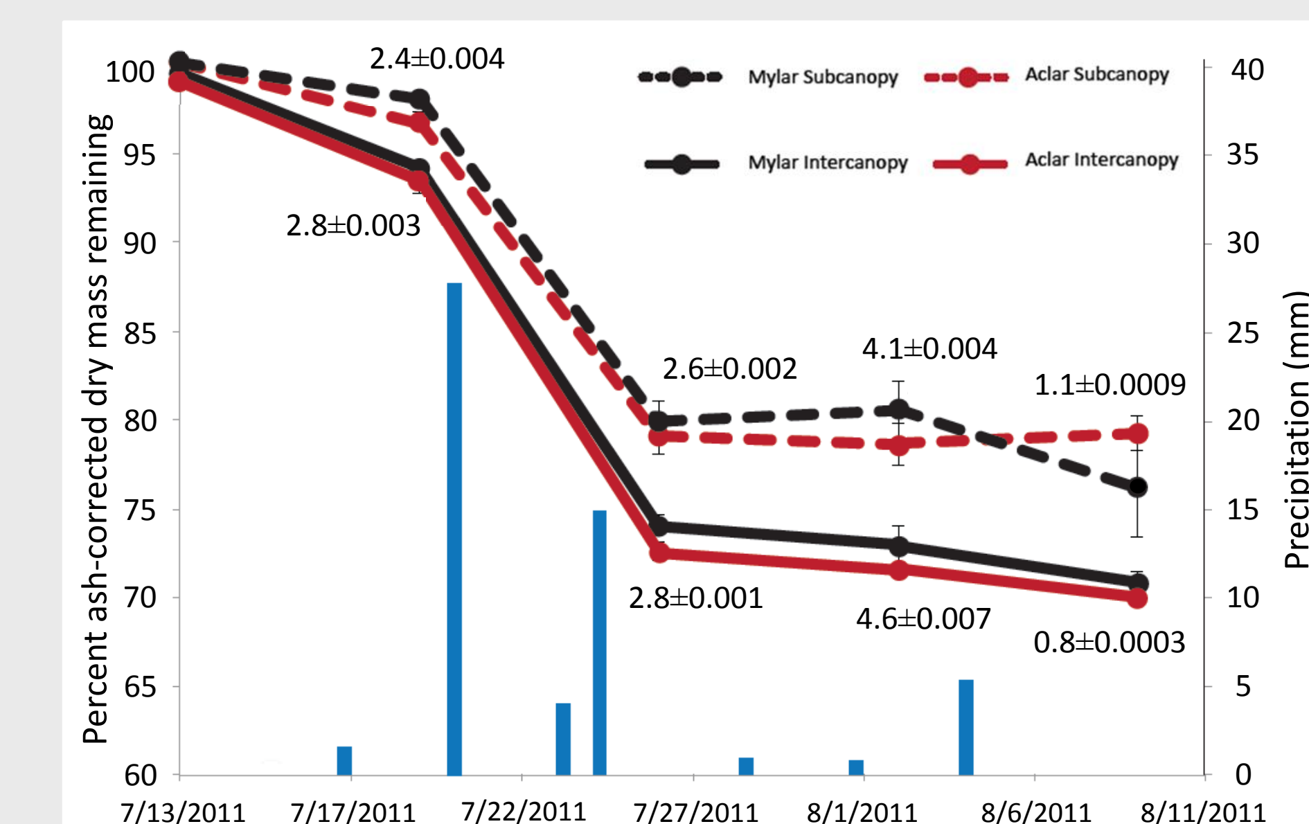
Figure 2 – Mean ( \pm 1 S.E.; n=5 ) ash-corrected mass loss (scaled so time 0 values start at 100% and represent initial litter mass). Numerical values associated with each harvest date indicate mean ( \pm S.E.) soil moisture in intercanopy and subcanopy placements. Bars represent the daily precipitation.
