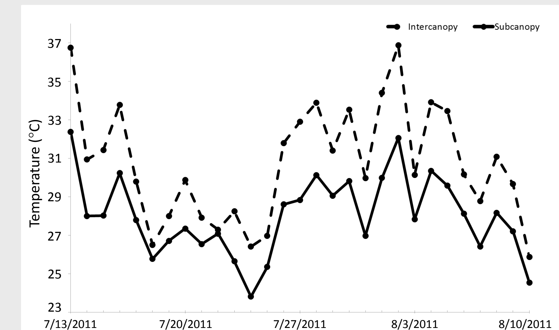
Figure 1 – Average daily temperature (monitored hourly) on bare soil in intercanopy and subcanopy zones.
