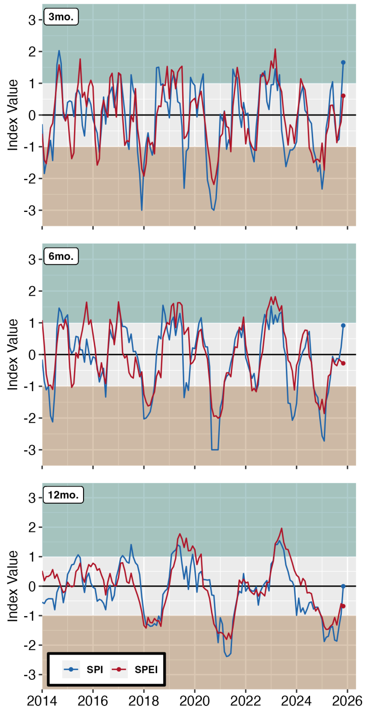
Figure 3: [Top-Left] Drought classification quadrant for the 12-month SPI and STI (Standardized Temperature Index). [Bottom-Left] Table showing 3-, 6-, and 12-month climate statistics for the Prescott National Forest. [Right] Time series plots of the 3-, 6-, and 12-month SPI and SPEI.
