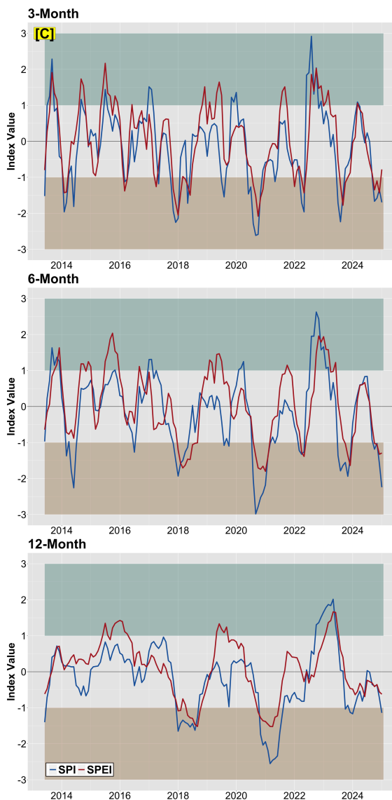
[A] Drought classification quadrant of the 12-month SPI and 12-month STI (Standardized Temperature Index). [B] Table showing 3-, 6-, and 12-month climate statistics for the Gila National Forest. [C] Time series plots of the 3-, 6-, and 12-month SPI and SPEI.
