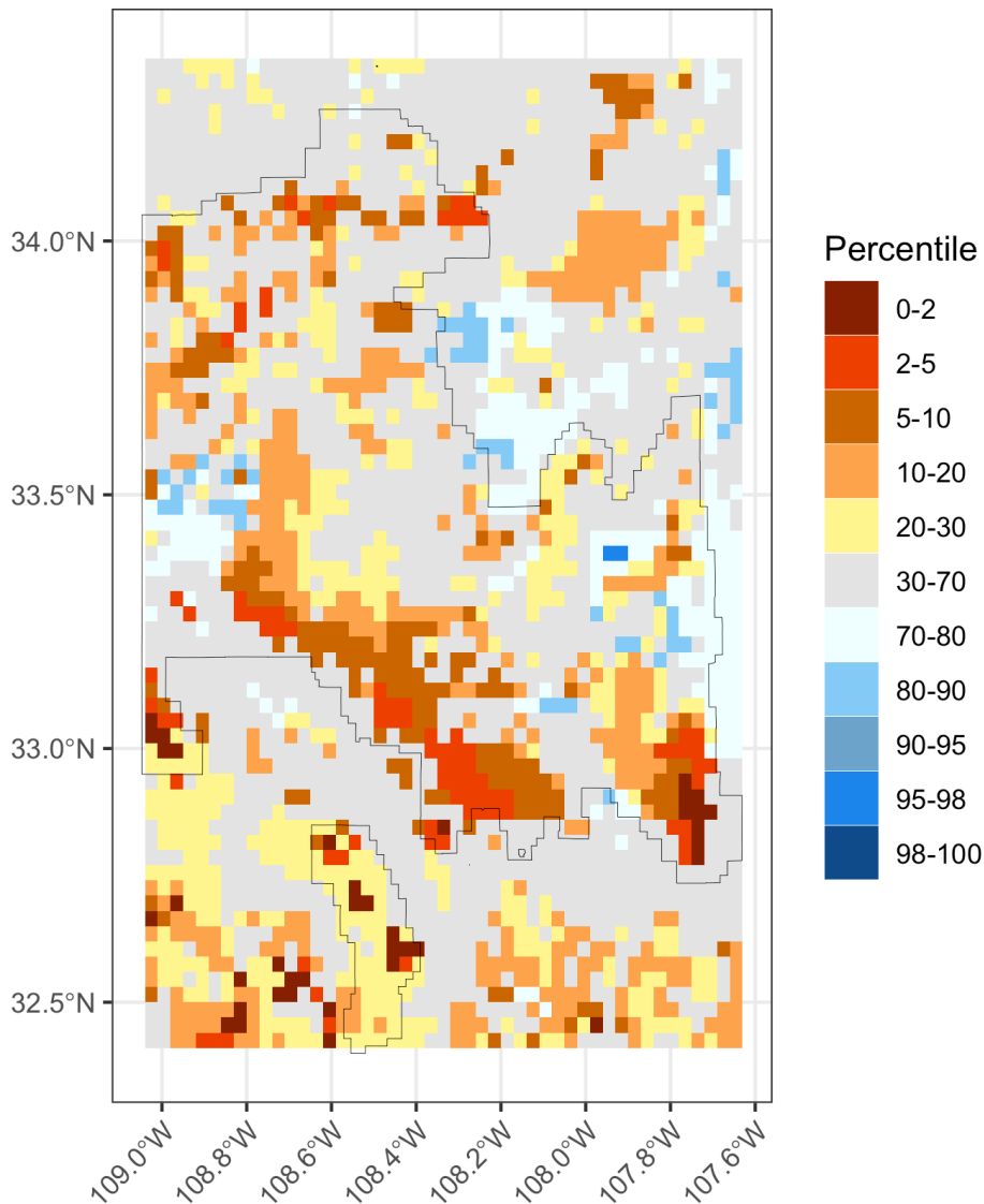
Figure 4: Integrated surface to 2 meter deep relative soil moisture estimate
