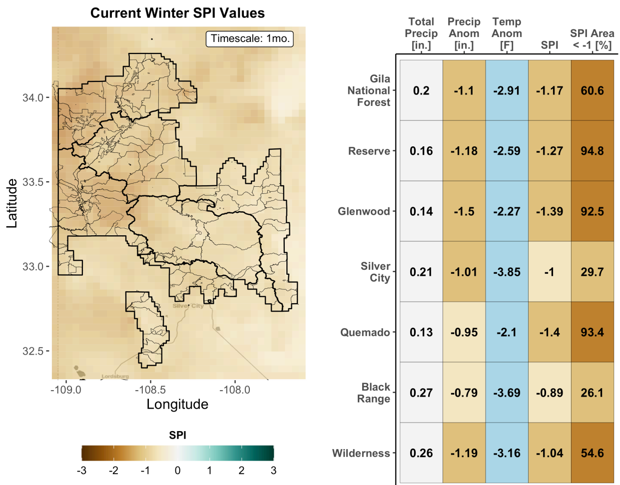
Figure 1: [Left] Gila National Forest Standardized Precipitation Index (SPI) values for Winter 2025 (January 1mo. timescale). [Right] Table summarizing climate statistics for Winter 2025 (January - January). Note: Season in progress - partial statistics being reported.
