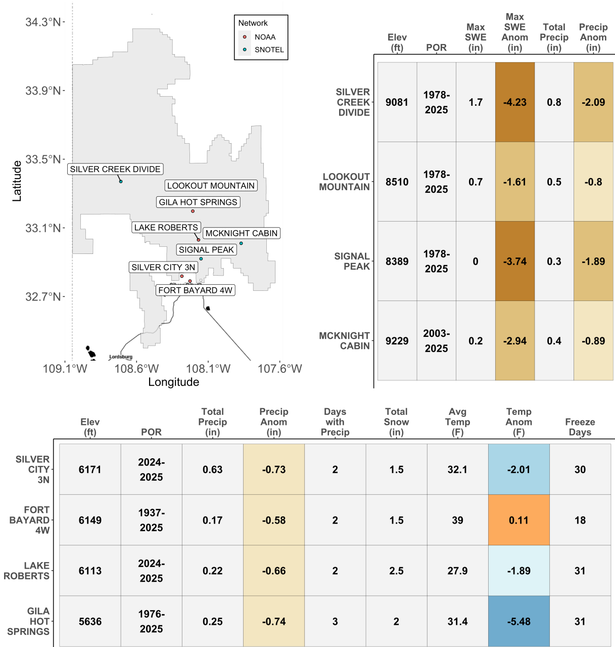
Figure 3: [Top-Left] Locations of NOAA and SNOTEL station(s) located within the report area boundary. [Top-Right] Table of SNOTEL station(s) statistics from 2025-01-01 to 2025-01-31. [Bottom] Table of NOAA station(s) statistics from 2025-01-01 to 2025-01-31.
