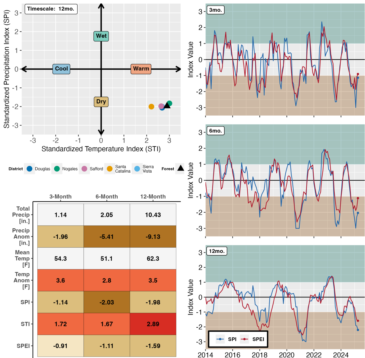
Figure 3: [Top-Left] Drought classification quadrant for the 12-month SPI and STI (Standardized Temperature Index). [Bottom-Left] Table showing 3-, 6-, and 12-month climate statistics for the Coronado National Forest. [Right] Time series plots of the 3-, 6-, and 12-month SPI and SPEI.
